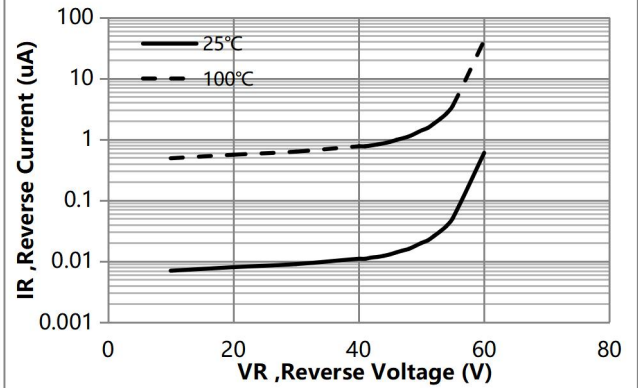
FIG.2 Reverse Characteristic (typ.)
