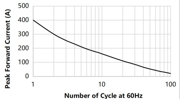
FIG4. Maximum Non-repitive Surge
